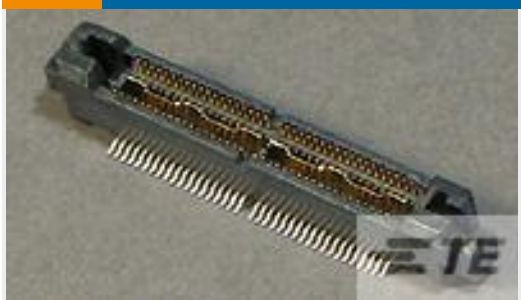
TE 产品编号 5767057-2 MICT,495,PLUG,076,PDNI
