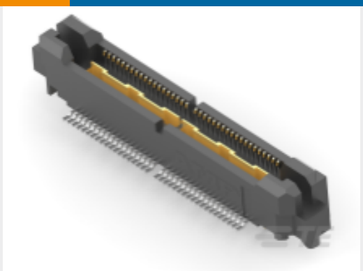
TE 产品编号 5767117-2 MICT,260,PLG,076,ASY,.025,PDNI
