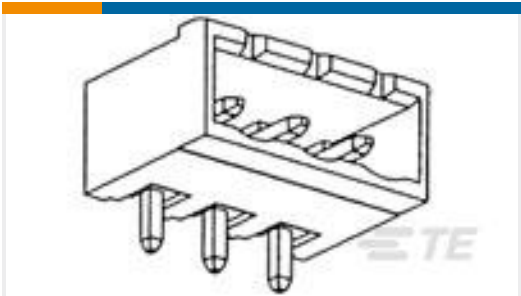
TE 产品编号796645-6 6POS 5.0MM CE R/A HDR,TRM BLK
