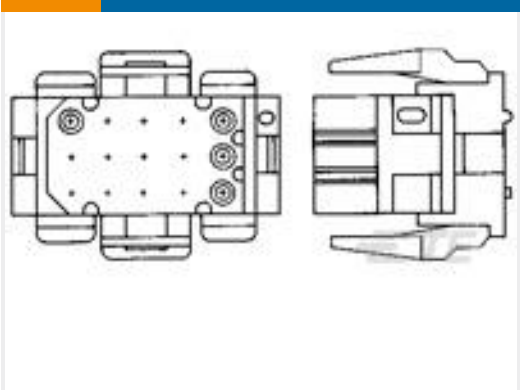
TE 产品编号1-640523-0 15P MR II PLUG HSG V0 RED
