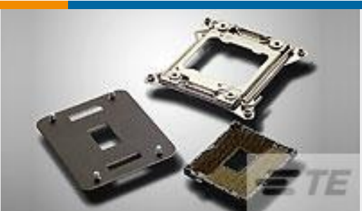
TE 产品编号1554653-1 SOCKET ASSY LGA2011, 0.38Au
