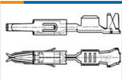
TE 产品编号1241858-2 MT3 REC 1.6 Contact SWS Sn
