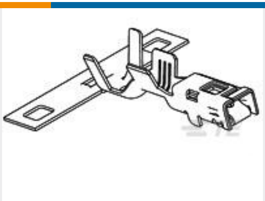
TE 产品编号1326032-5 2.8MM RECP,SEAL,14AWG
