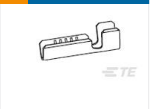
TE 产品编号160644-3 SPLICE 20-15 AWG .016 TPBR
