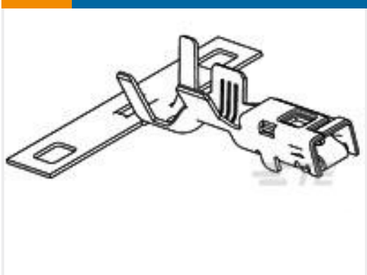
TE 产品编号1326032-3 2.8MM RECP,SEAL,18AWG
