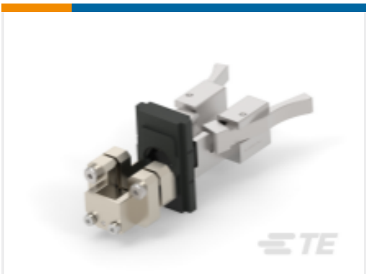
TE 产品编号1-528041-3 DIE SET SHIELD CRIMP HVP800 90DEG.35SQMM
