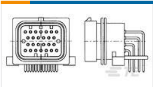
TE 产品编号9-6437287-8 SUPER SEAL 26POS CAP ASSY H AU
