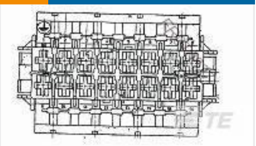
TE 产品编号927669-2 STANDARD TIMER HOUSING 16POS
