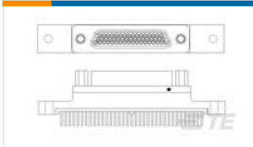
TE 产品编号2204452-1 MULTI-BEAM HD R/A PLUG 15S+6P+2LP+15S
