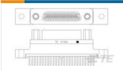
TE 产品编号1-5767007-1 MICT,260PLUG,152,ASSY,.025,REC
