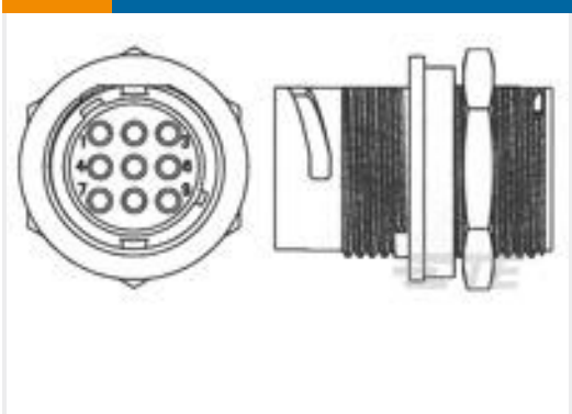
TE 产品编号1445816-1 RECPT,11-9,FLNG MT,STD KEY
