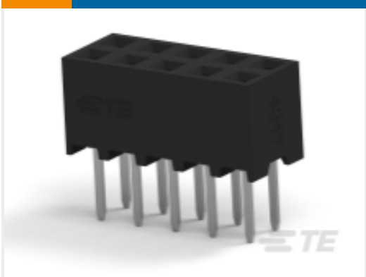
TE 产品编号1-2314820-0 10P,2MM,B-B,REC,DRVT,2.7,0.1AU,TB
