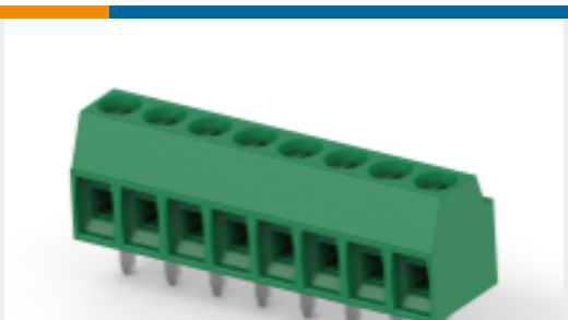
TE 产品编号1546551-8 8P,STRAIGHT,SIDE ENTRY,3.5MM
