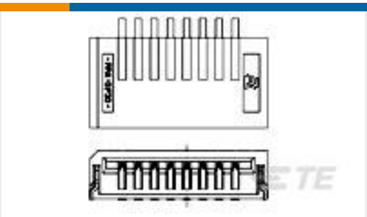
TE 产品编号1735360-8 1mm FFC SMT H BOTTOM CONTACT ASSY, 8P
