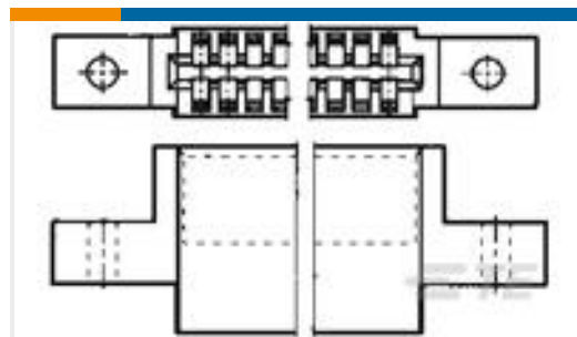
TE 产品编号2-583718-7 TW-LEAF CRP HSG 32 POS 100C/L
