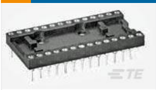
TE 产品编号1571550-6 520-AG12D-LF=500 DIP,PCB,SN/SN
