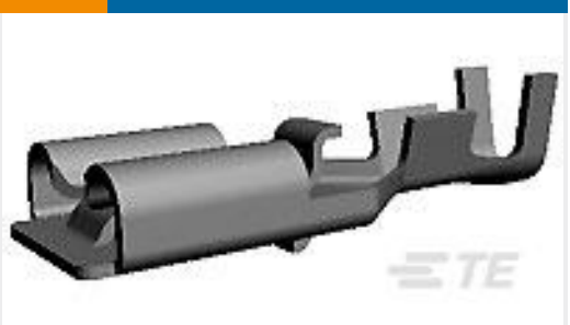
TE 产品编号179973-6 PL EX 250 REC 22-18 PTPCOPPER-ALLOY
