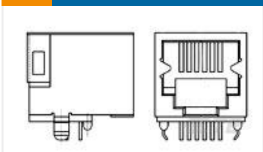
TE 产品编号1734723-6 RJ11,6P6C,SINGLE,DIP, 15u" Au, Reel
