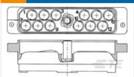
TE 产品编号1604798-2 ASY,RCPT,PWB MT,12 POS
