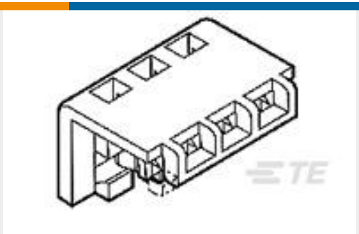
TE 产品编号1-643067-8 18P MTA156 MOLDED COVER
