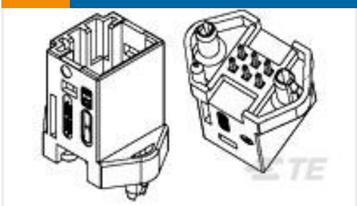
TE 产品编号1379816-3 6pos MQS .63 header 180deg
