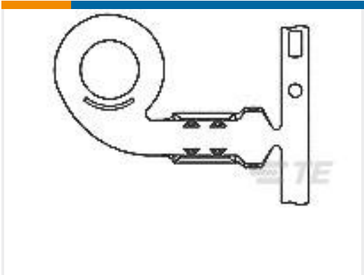
TE 产品编号9-226619-1 GND FLAG TERMINAL, LF PLTG
