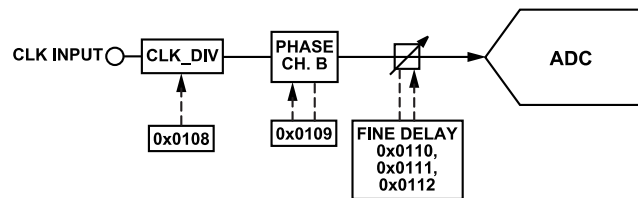
Figure 67. Clock Divider Phase and Delay Controls
