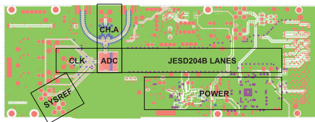
Figure 128. Recommended PCB Layout for the AD9699
