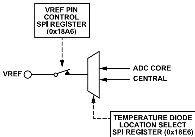
Figure 72. Register Controls to Output Temperature Diode Voltage on the VREF Pin
