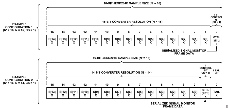
Figure 99. Signal Monitor Control Bit Locations
