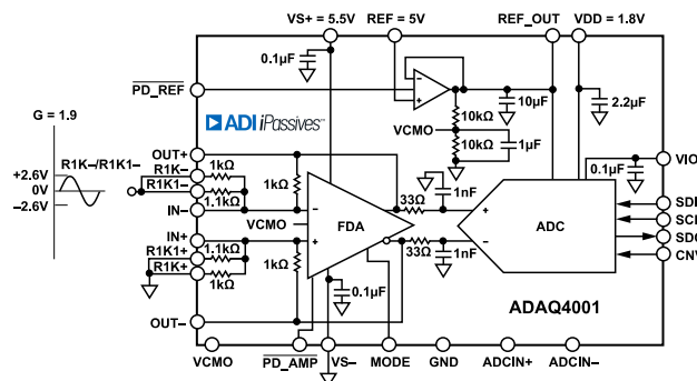
Figure 44. Single-Ended to Differential Configuration with G = 1.9
