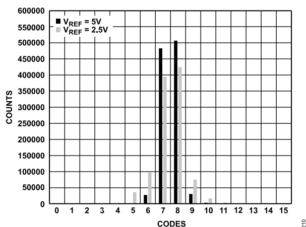
Figure 6. Histogram of a DC Input at the Code Transition, V_{REF} = 2.5\text{ V} and V_{REF} = 5\text{ V}
