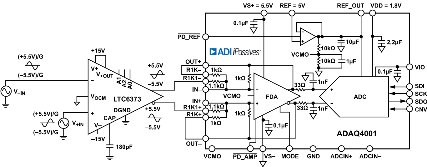
Figure 51. LTC6373 Driving ADAQ4001 (G = 0.454)
