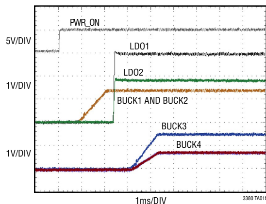
Start-Up Sequence
