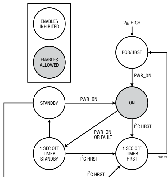
Figure 5. LT3380 Operating Mode State Diagram
