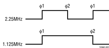
Figure 3. Phase Settings Full- and Half-Speed Buck Clock
