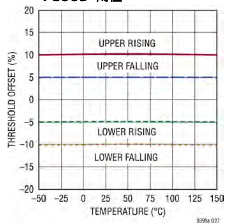
PGOOD 阈值
